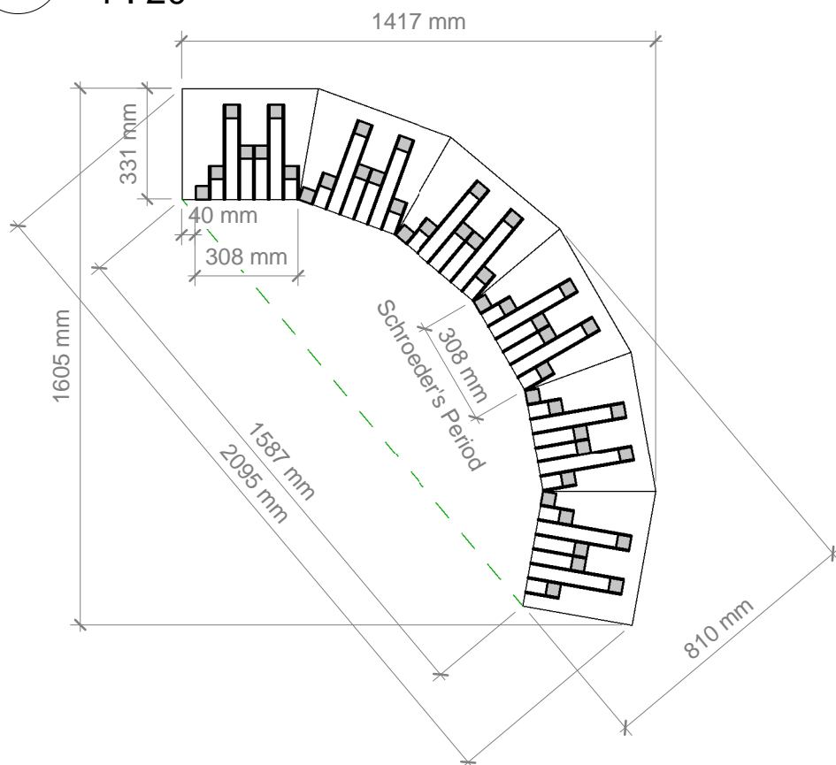
2 Plan view 1 : 20
