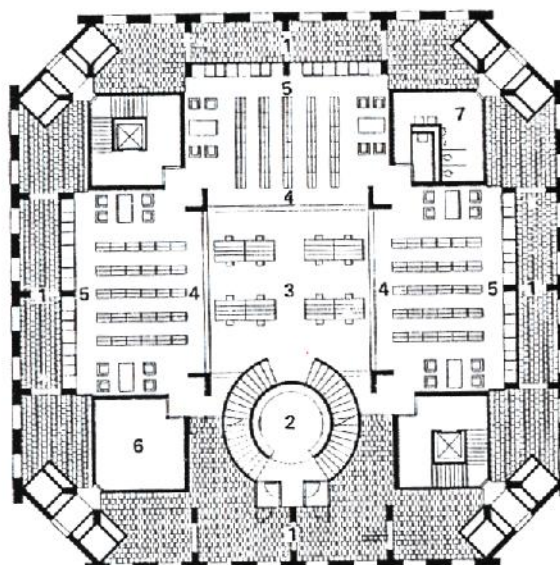
1 階平面図. First-floor plan.
