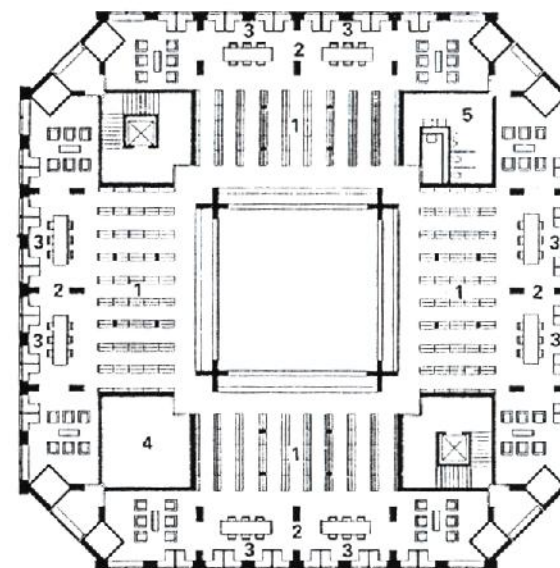
3 階平面図. Third-floor plan.
